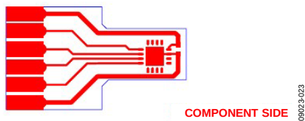
Figure 22. ADT7320FBZ Component Side (Layer1)
