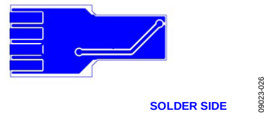
Figure 26. ADT7420FBZ Solder Side(Layer 2)
