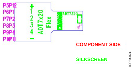
Figure 24. ADT7320FBZ Silkscreen
