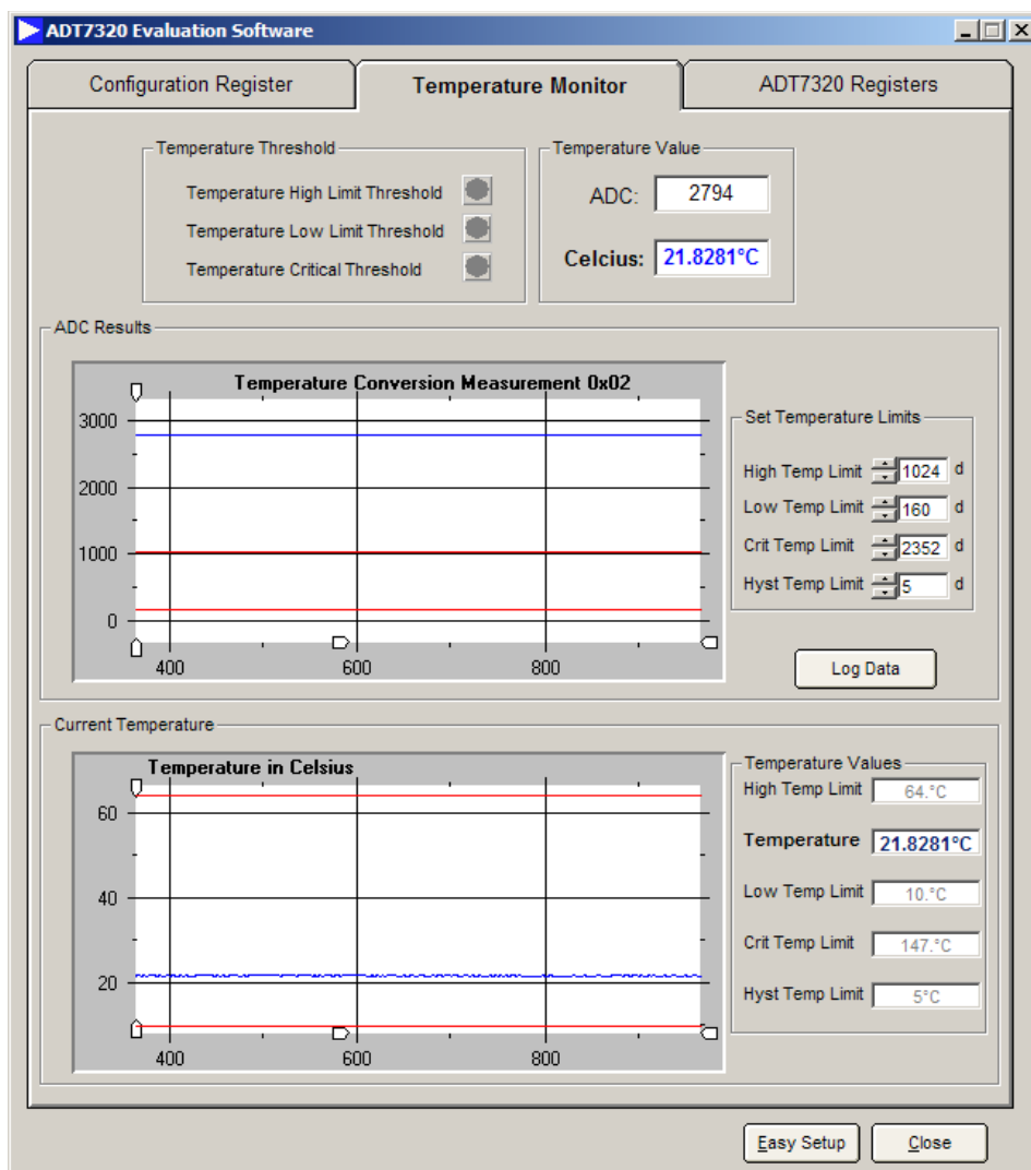
Figure 8. Temperature Monitor
