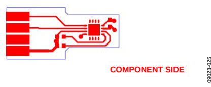
Figure 25. ADT7420FBZ Component Side(Layer1)
